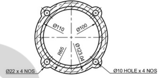
SECTION B-B (1:2.5)
